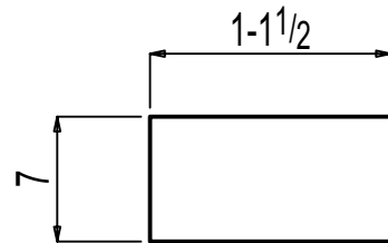
ONE SHIM PLATE F-08.02M2
