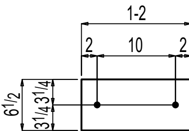
ONE LEVELING PLATE F-08.02LP2
