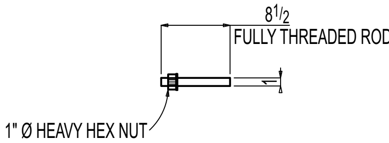
16 THREADED RODS F-08.02M7
