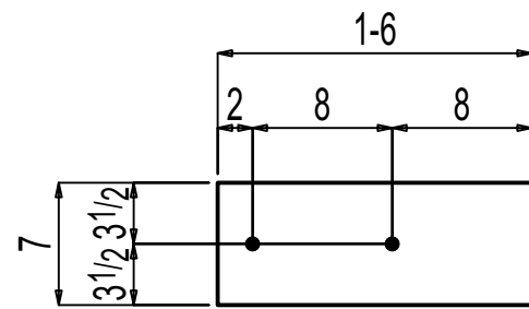
ONE LEVELING PLATE F-08.02LP1
