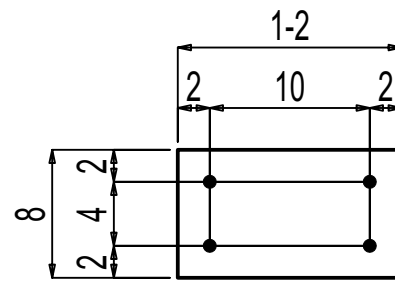
ONE LEVELING PLATE F-08.02LP3
