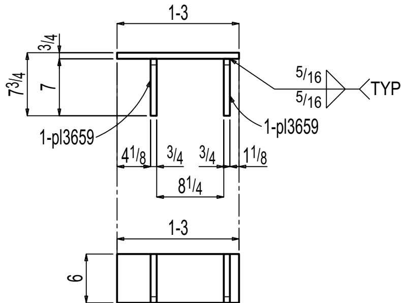
ONE PLATE F-08.02M3
