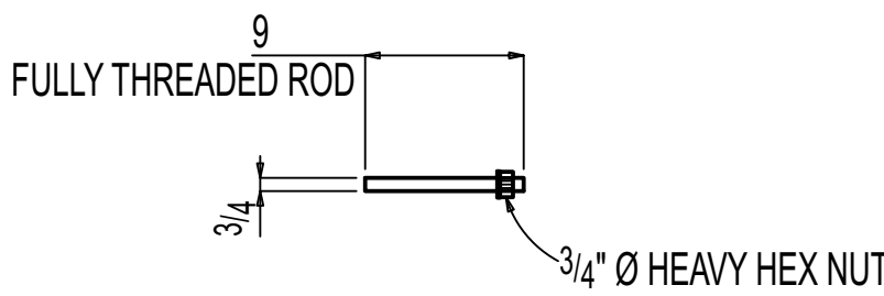
4 THREADED RODS F-08.02M5
